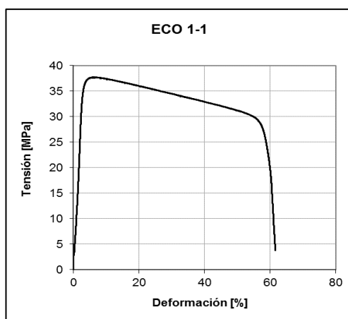
Figure 1. a) Stress-Strain curve and b) SEM image for ECO 1 solder.
