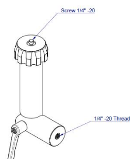
TBMA1C-PAT, shaft
